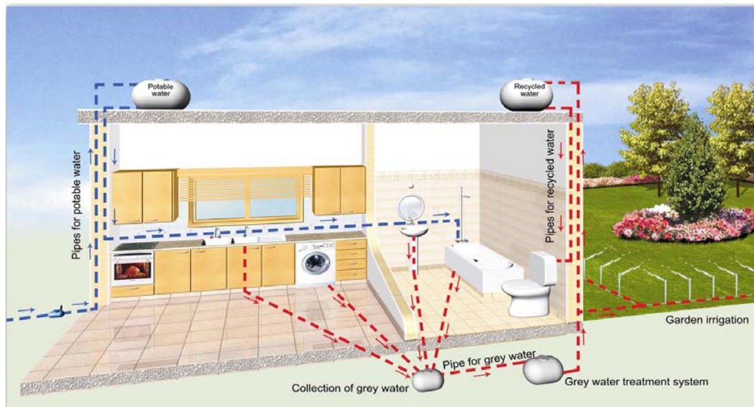
Figure 10 – Grey water reutilization system in Cyprus
