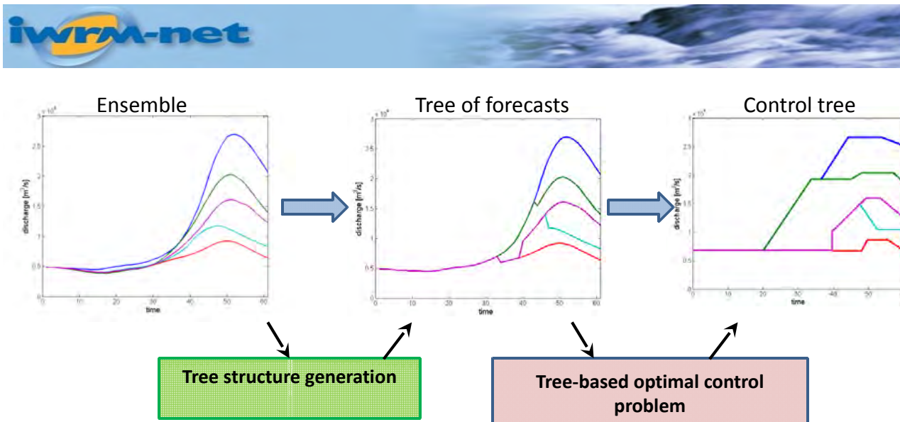
Figure 49: Scheme of the generation of a control tree from an ensemble forecast
