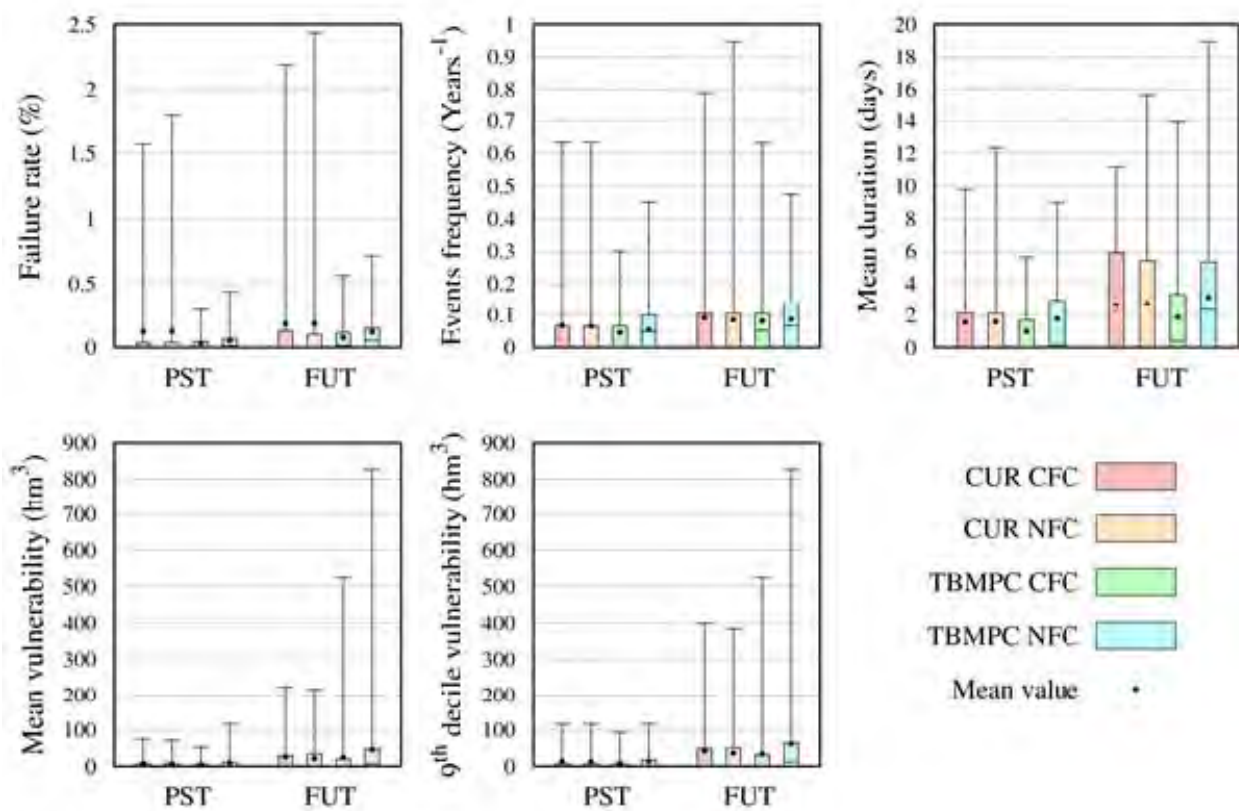
Figure 61: Performance indicators for the 2 nd high-flow threshold (Orange) calculated from 7 GCMs scenarios in present (PST) and future (FUT) time for 4 management adaptations.
