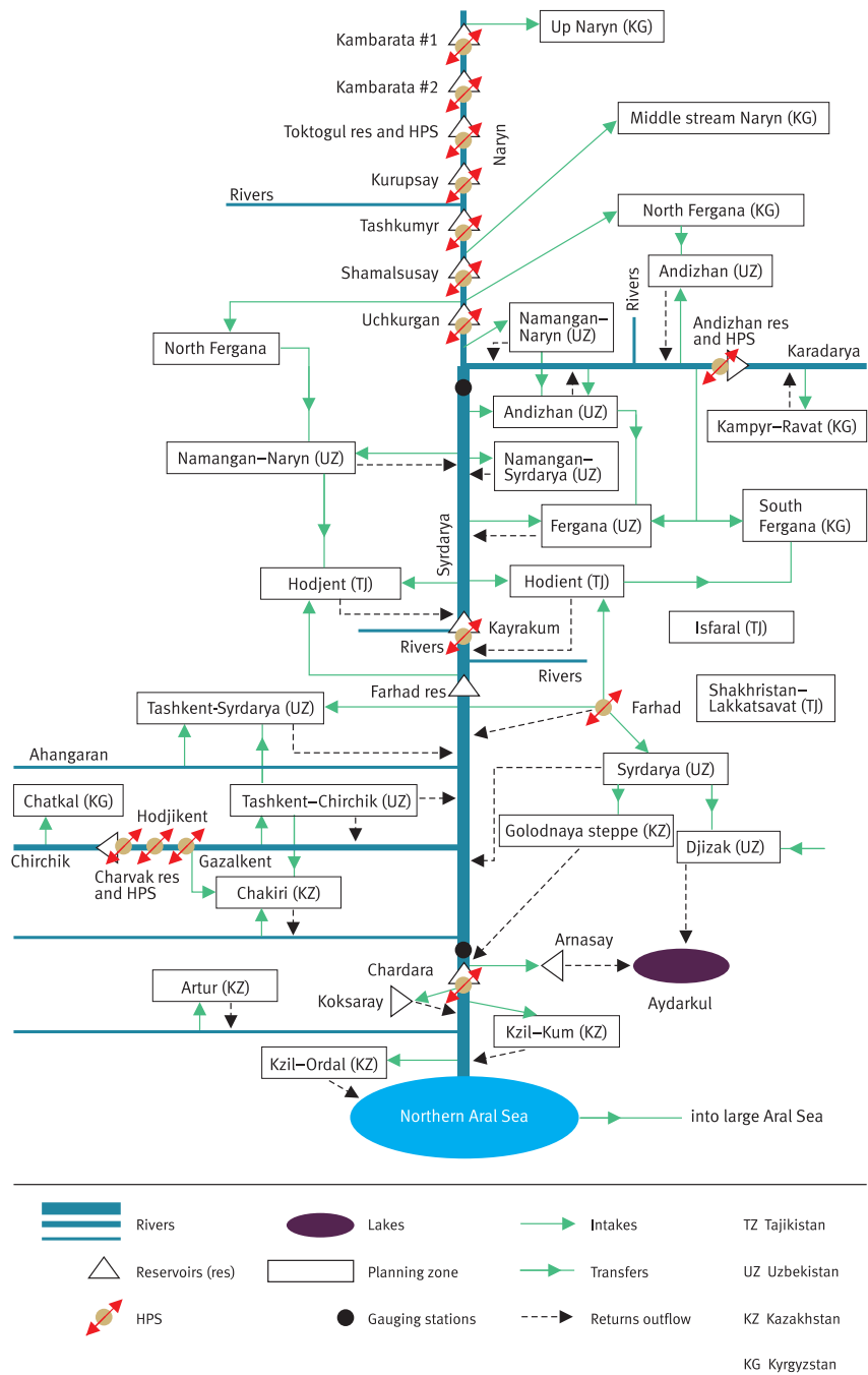
Figure 22. Schematic diagram of the Syrdarya River Basin
