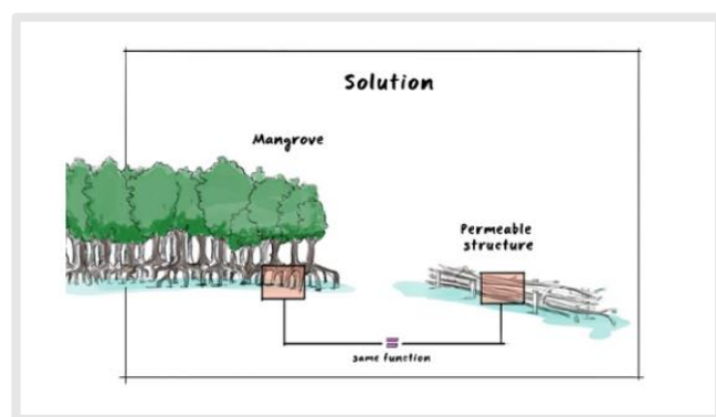
Permeable dams mimic the structure of mangrove root systems to trap sediment and dampen waves © EcoShape
