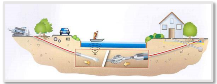
Horizontal Directional Drilling (HDD) – Source: WWF Hungary
